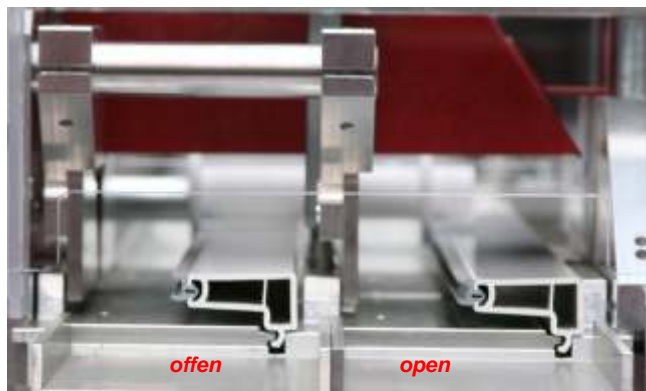
Spannsituation/ Glassimulation
