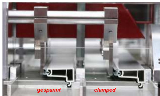
Clamping situation/ glass simulation unit
